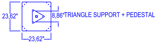
CONCRETE ANCHORAGE
